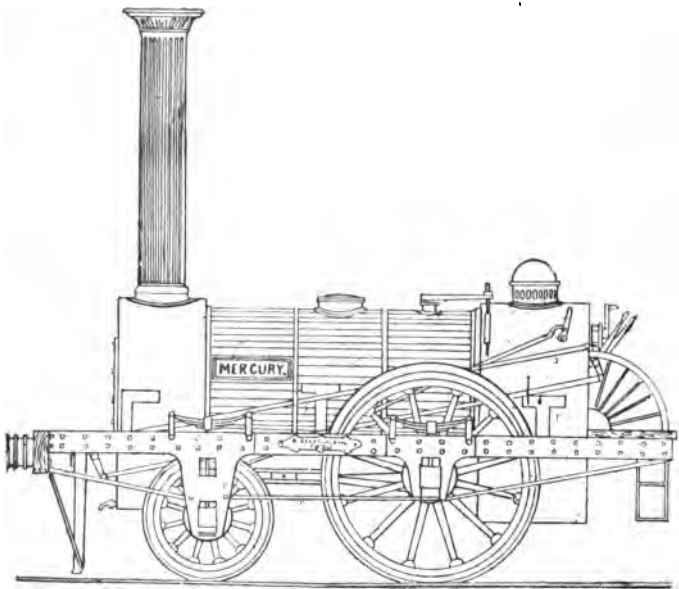
Fig. 21.—"Mercury," No. 11, Liverpool and Manchester Railway, December, 1830.
